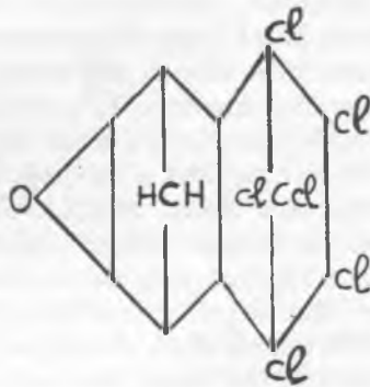
Dieldrinas
