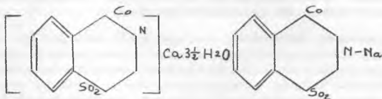
Kalcio sacharinas
